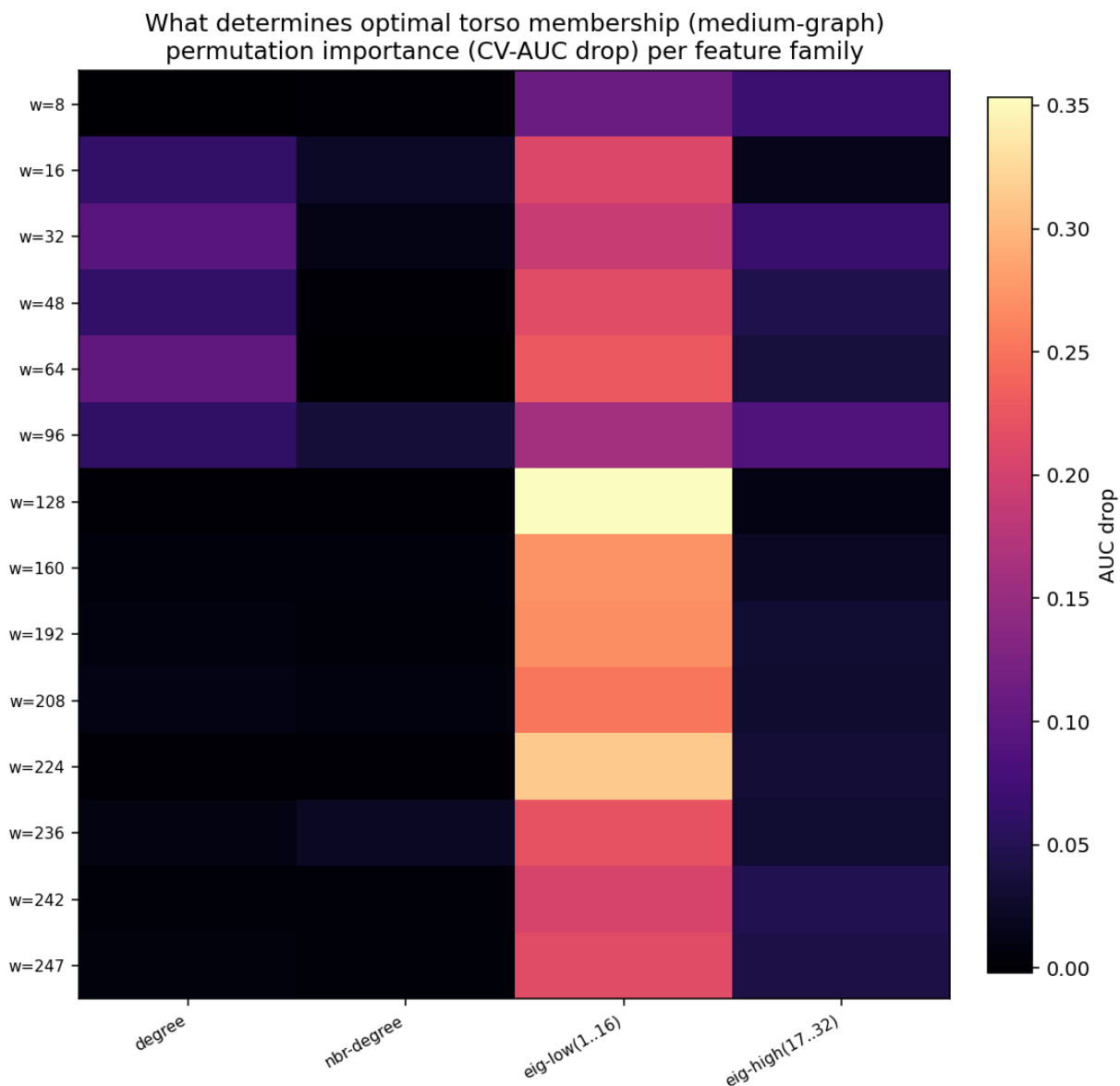
Figure 15: GBDT permutation-importance map for medium-graph. Unlike small (Fig. 13.7), there is no local regime: the low-eigenvector column is the sole bright stripe across the entire 0–248 width spectrum, peaking near w = 128 — optimal torso membership is globally/spectrally determined at every resolution.
